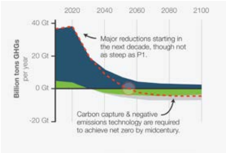
Scenario S1. Steep reductions in the '20s and '30s
